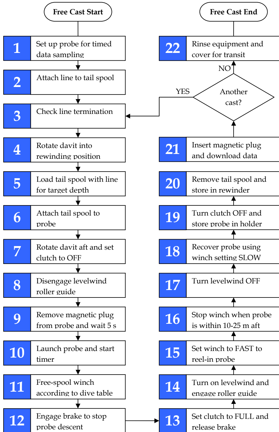
Figure 9 Flow chart for free casts.
