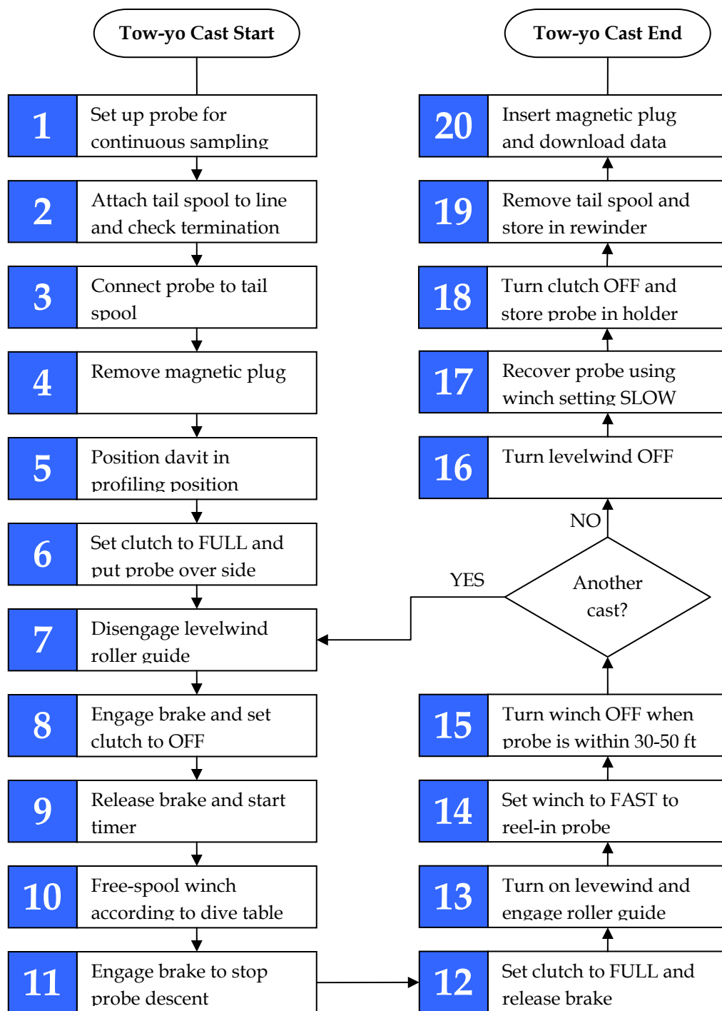
Figure 8 Flow chart for tow-yo casts.
