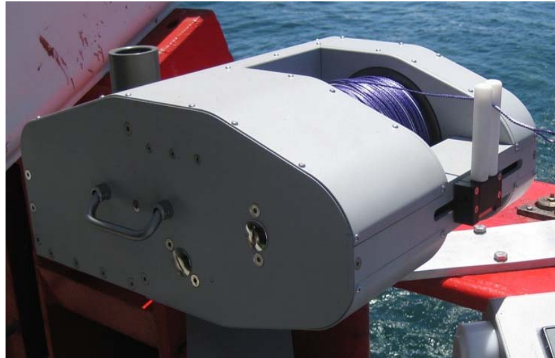
Figure 1 UnderwaySV winch and levelwind.
