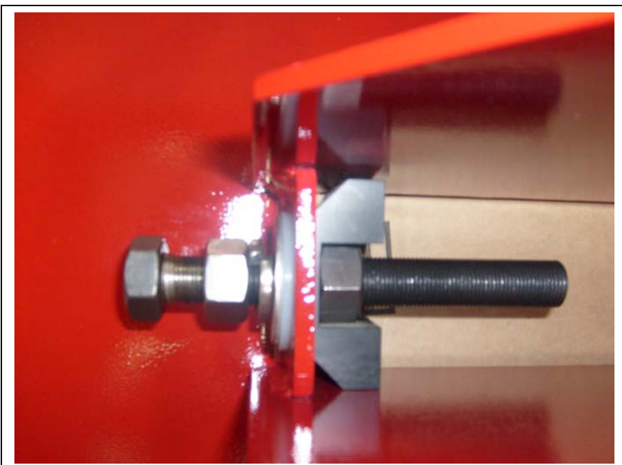
Inner Compression Bolt
